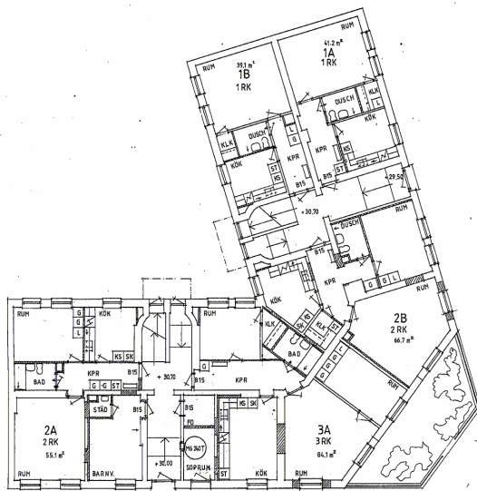
BOTTENPLAN
